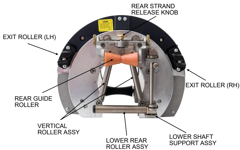
Fig. 32, Rear View
