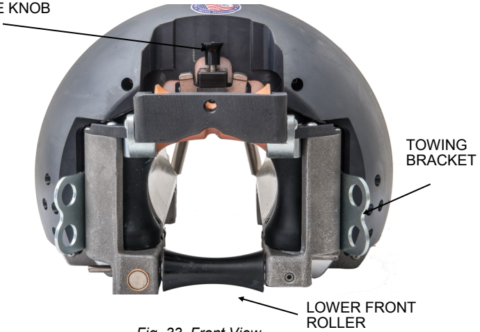
Fig. 33, Front View
