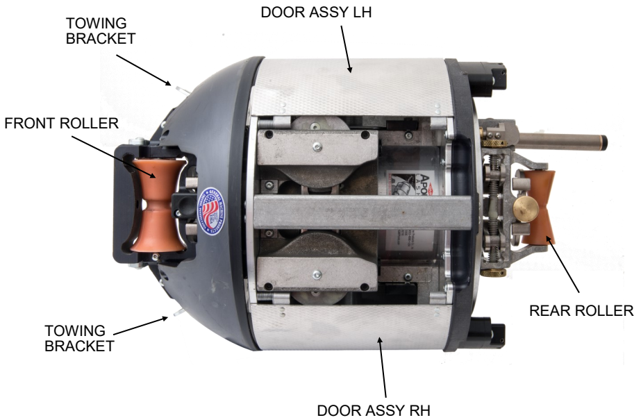
Fig. 34, Top View
