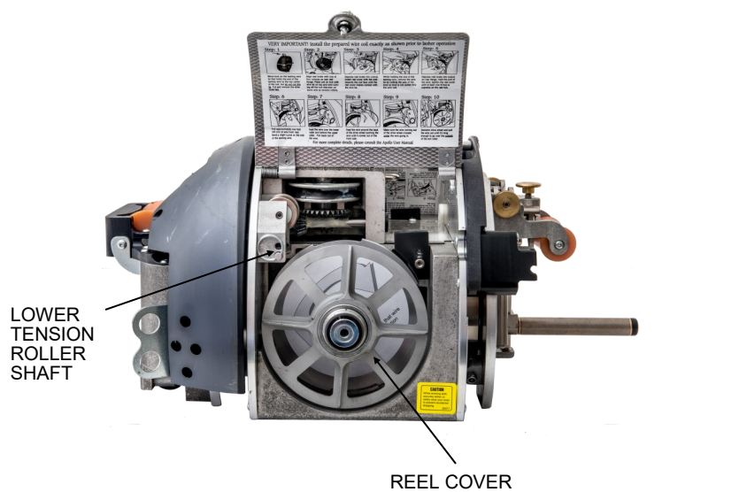
Fig. 31, Side View
